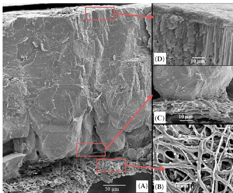
Figure 1. Scanning electron microscopy of the highly ordered structure of the chicken eggshell
