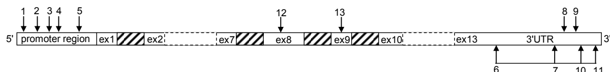
Figure 1. Schematic overview of the SNPs detected in PPARGC1A ; numbered arrows indicate detected SNPs; connected arrows represent linked SNPs; striped box: intron
