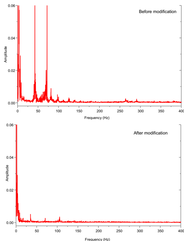
Figure 4. Vibration amplitudes at different frequencies before and after modification of the milking unit
