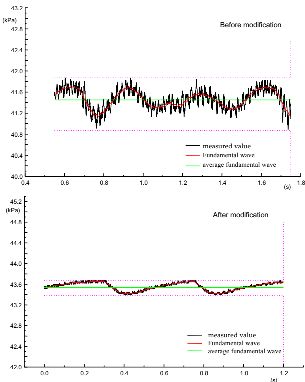
Figure 3. Vacuum stability in the air line before and after modification of the milking system
