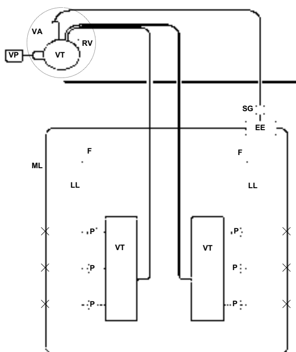
Figure 1. Schematic representation of the redesigned milking system
